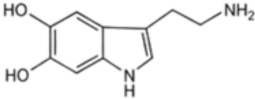
Serotonin
