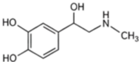
Epinephrine
